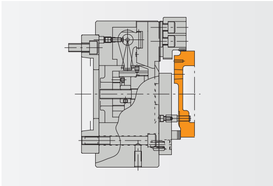
●ヨーク YOKE
